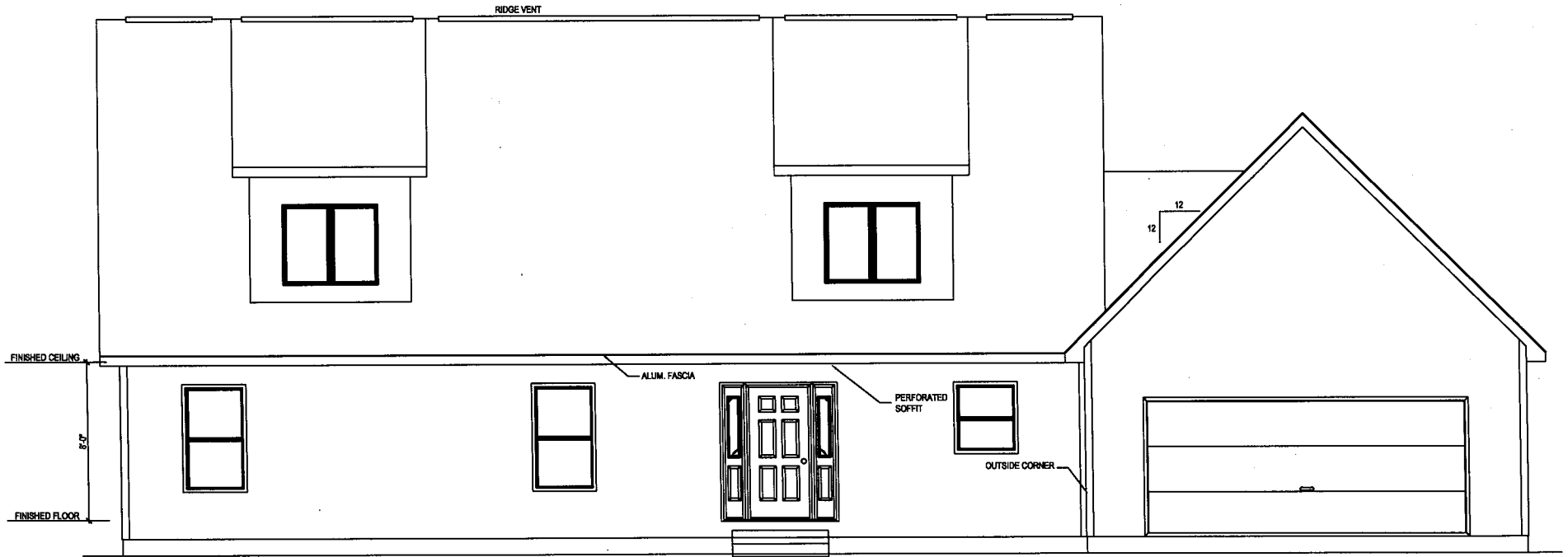
FRONT ELEVATION
