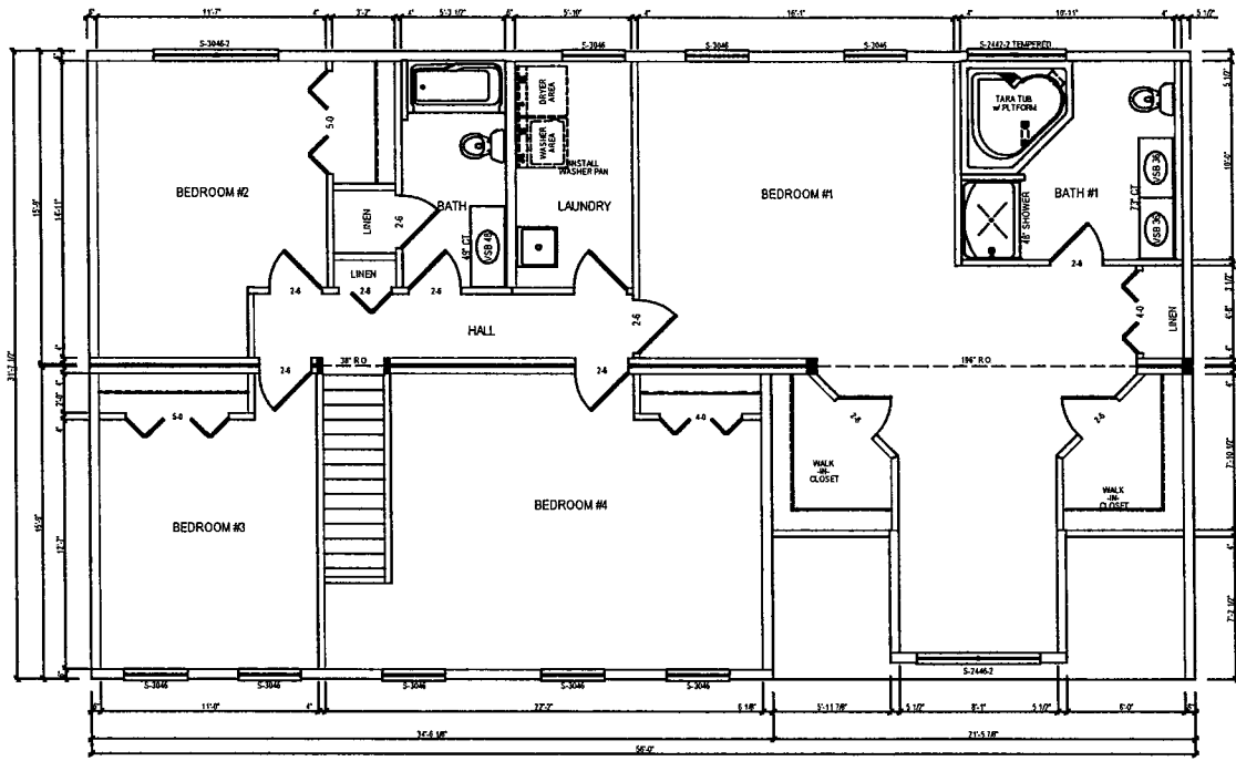
SECOND FLOOR PLAN 8'-0" CEILINGS
