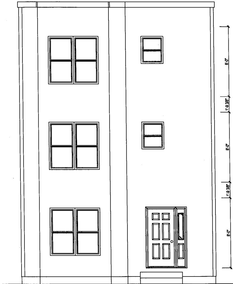
FRONT ELEVATION
