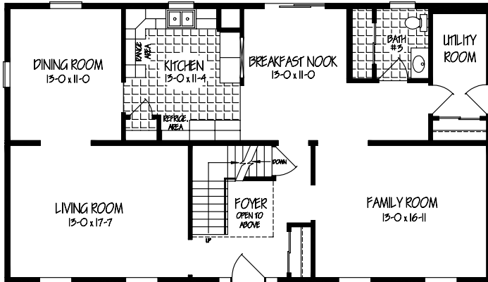
JAMESTOWN - II 27-6 x 48-0 FIRST FLOOR
