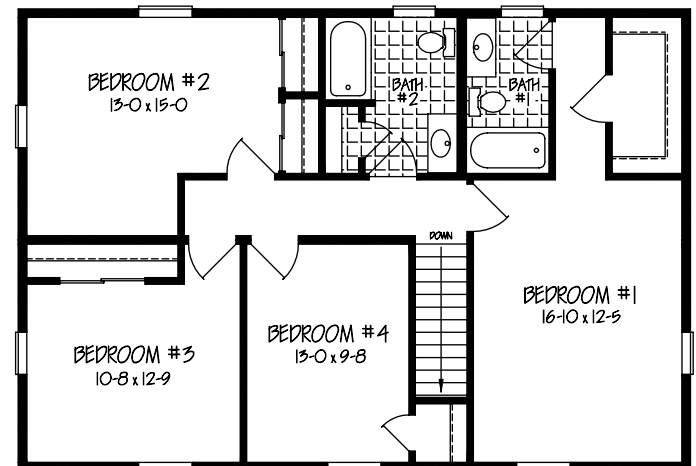
CLARKSBURG - III 27-6 x 40-0 SECOND FLOOR
