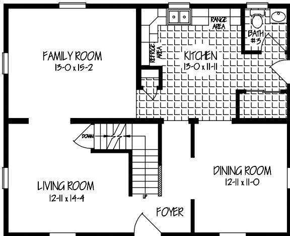
CLARKSBURG - II 27-6 x 34-0 FIRST FLOOR
