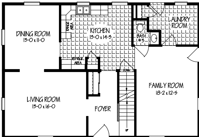
CLARKSBURG - III 27-6 x 40-0 FIRST FLOOR
