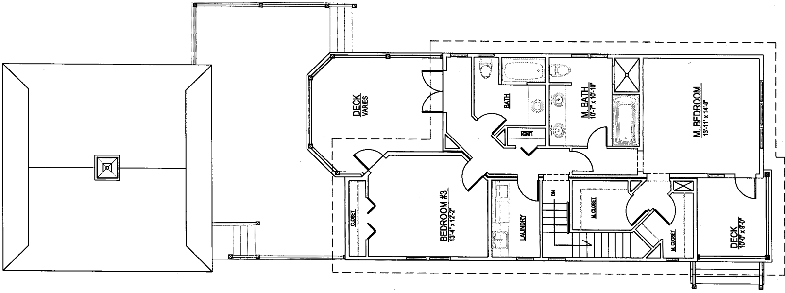
2nd. FLOOR PLAN SCALE: 1/4" = 10' FOOT
