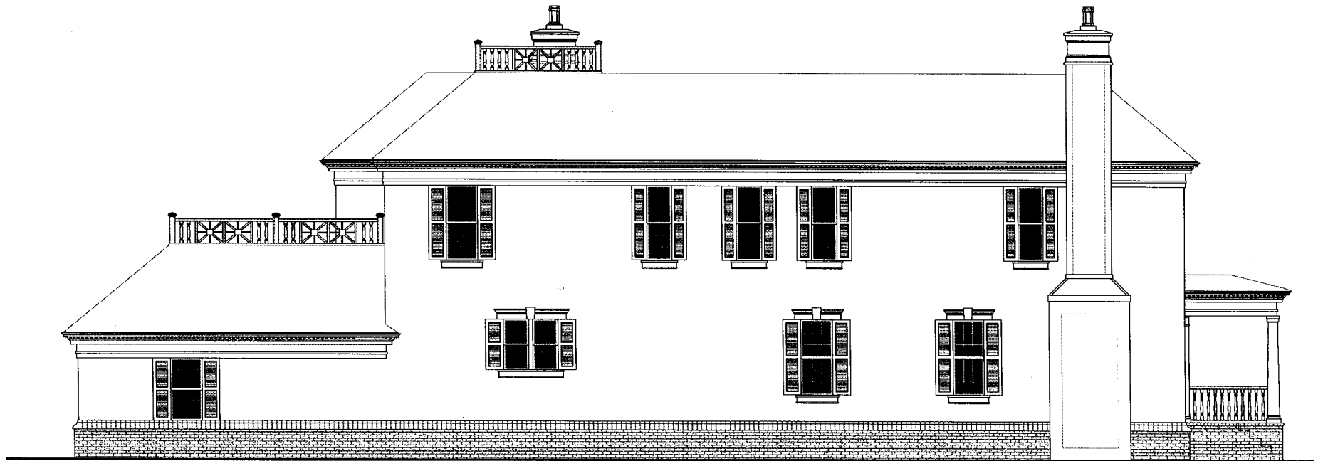
LEFT ELEVATION, FACING
