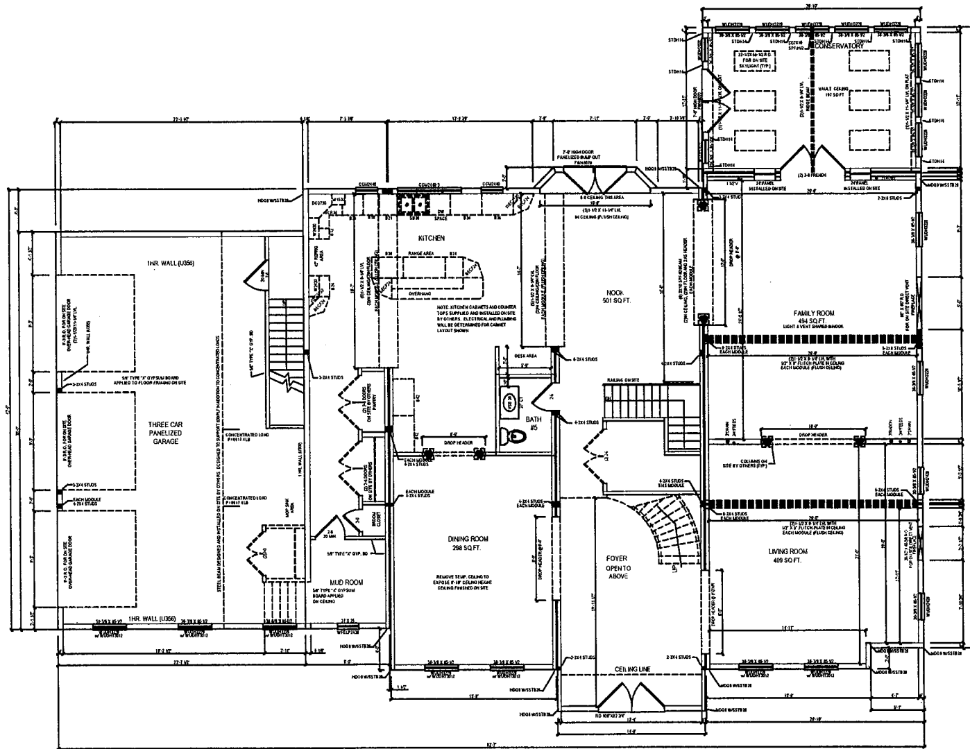
FIRST FLOOR PLAN 7'-0" CEILING
