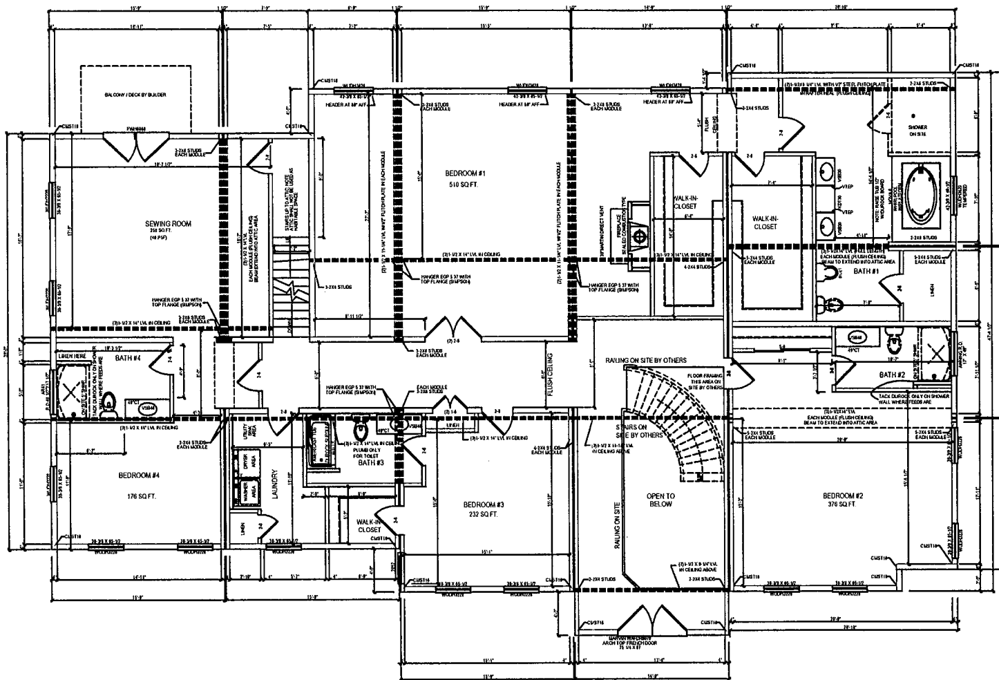
SECOND FLOOR PLAN 8'-0" CEILINGS
