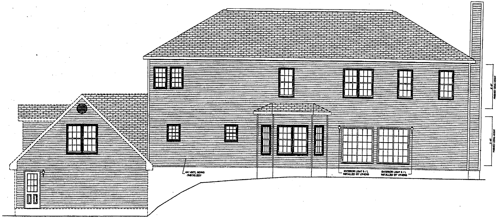
REAR ELEVATION
