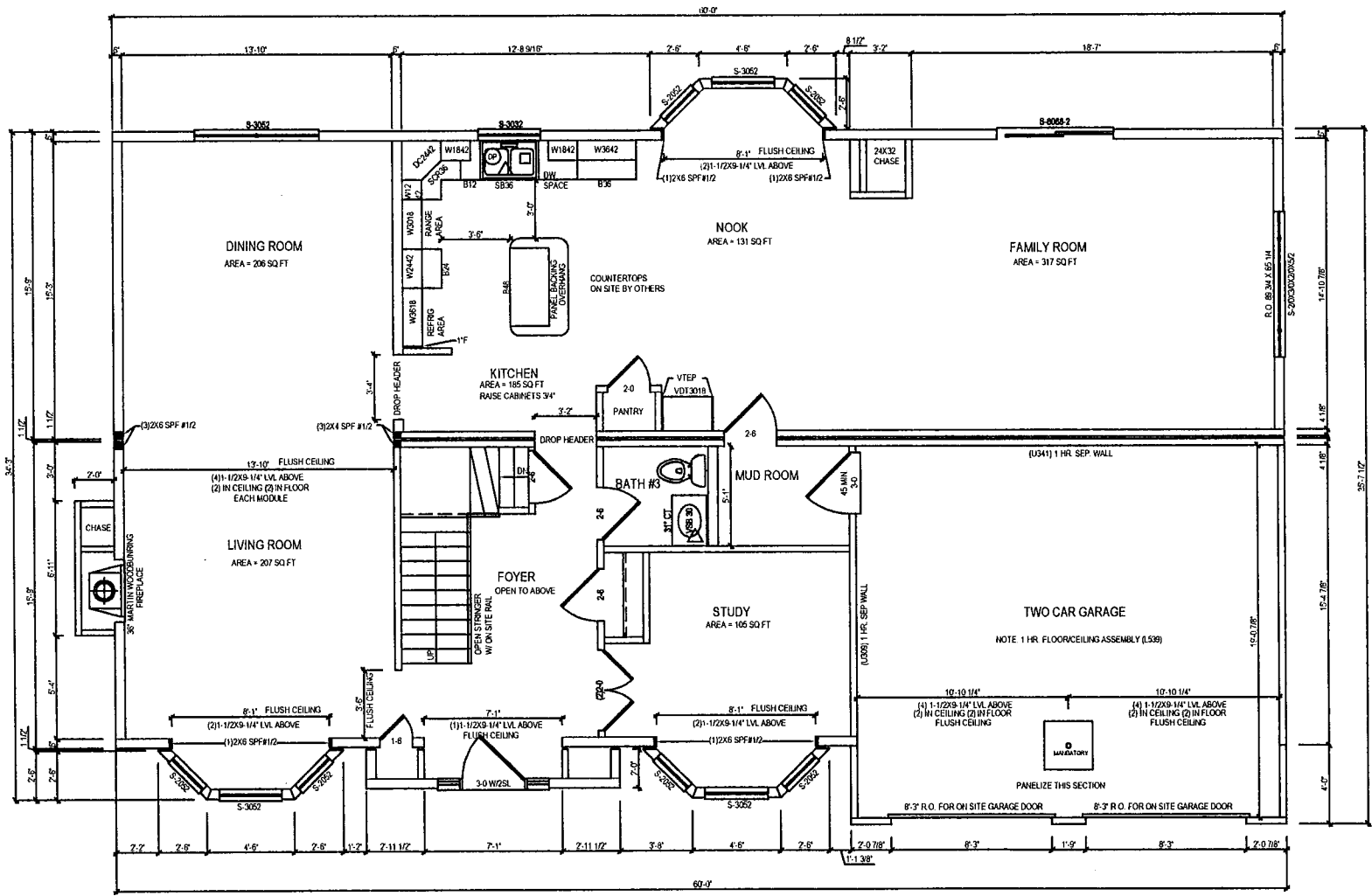
FIRST FLOOR PLAN 9'-0" CEILINGS
