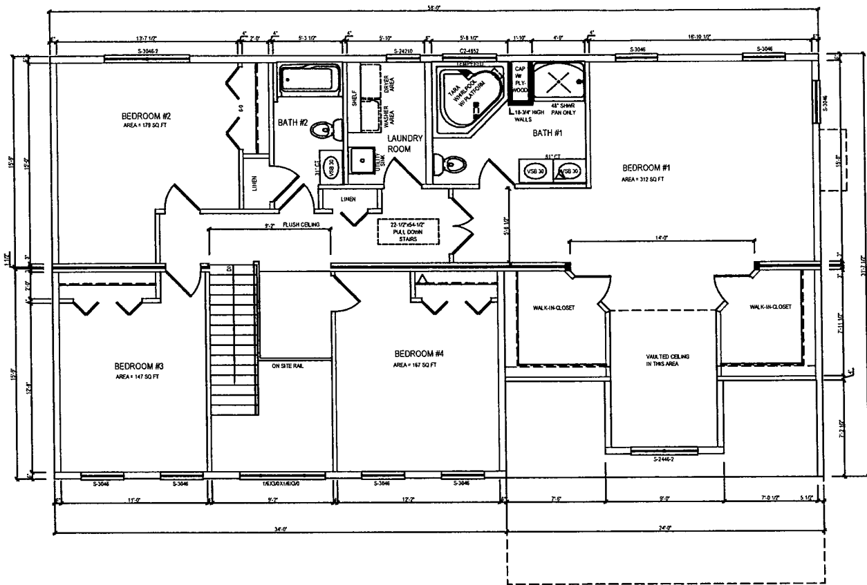
SECOND FLOOR PLAN 8'-0" CEILINGS
