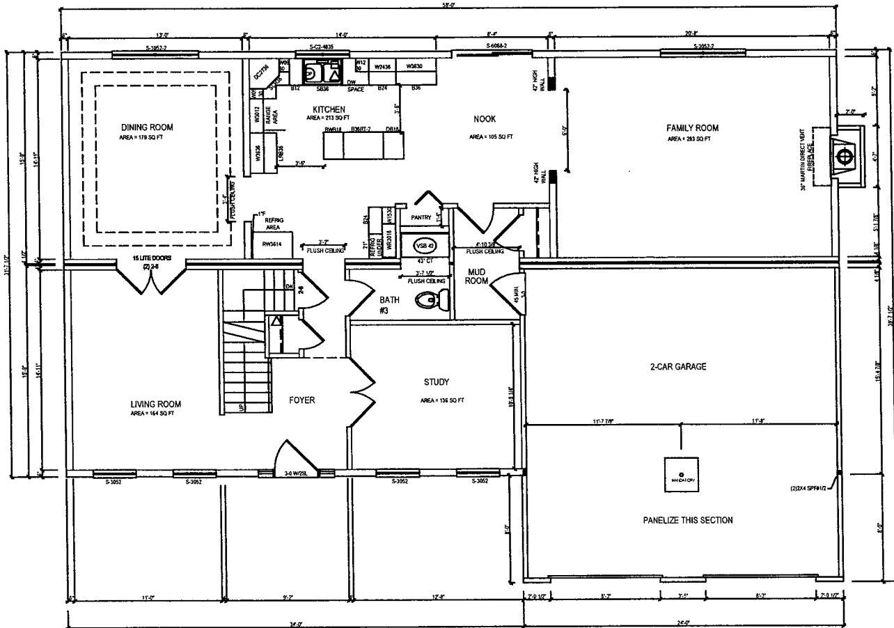
FIRST FLOOR PLAN 9'-0" CEILINGS
