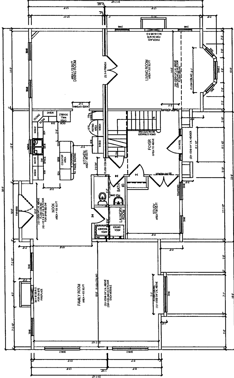
FIRST FLOOR PLAN S.P. CEILING
