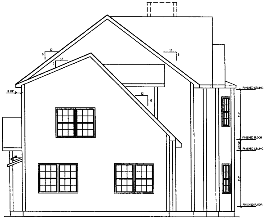
LEFT ELEVATION
