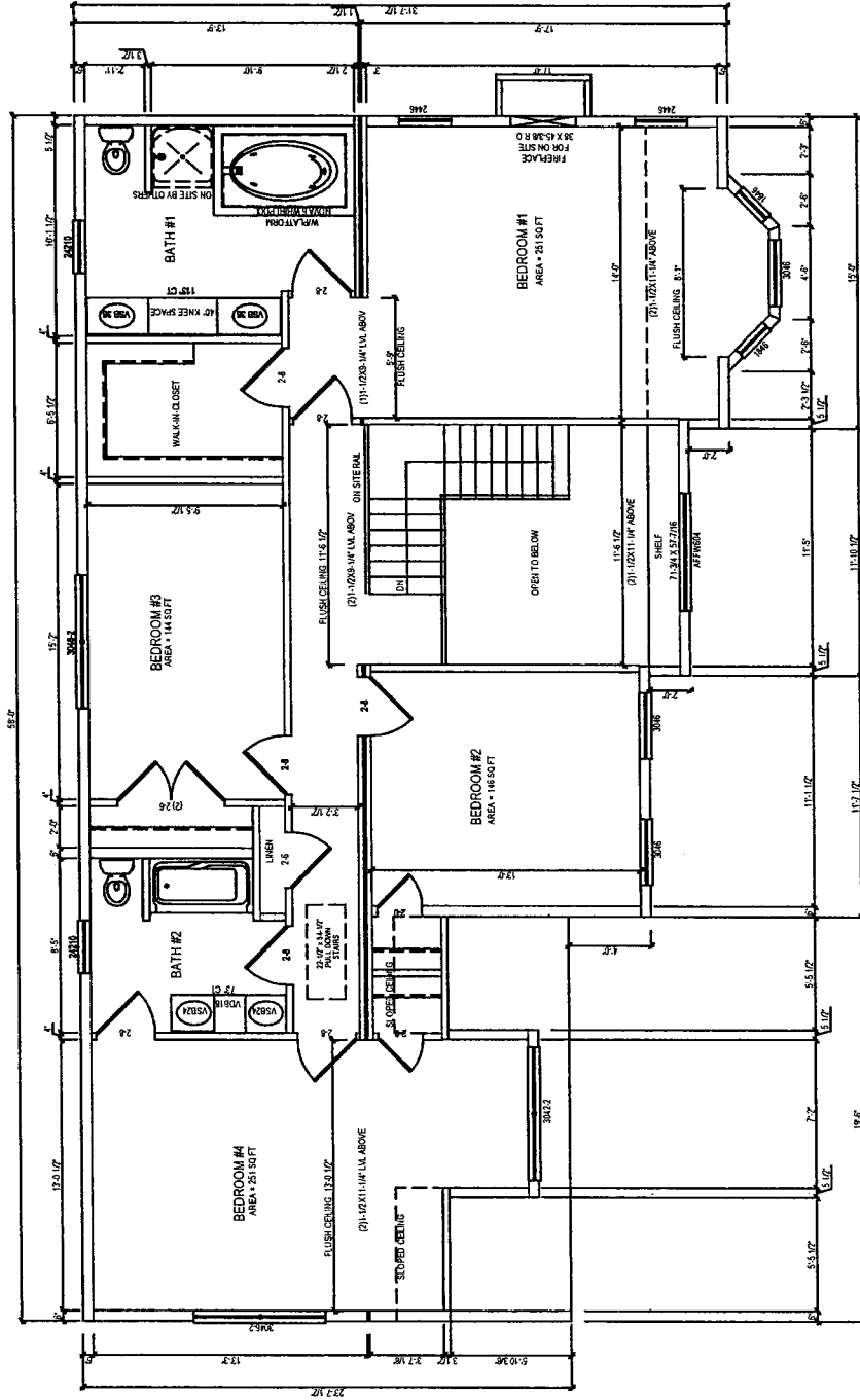
SECOND FLOOR PLAN 8'-0" CEILINGS
