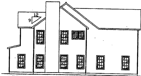
LEFT ELEVATION SCALE 3/16" = 1'-0"
