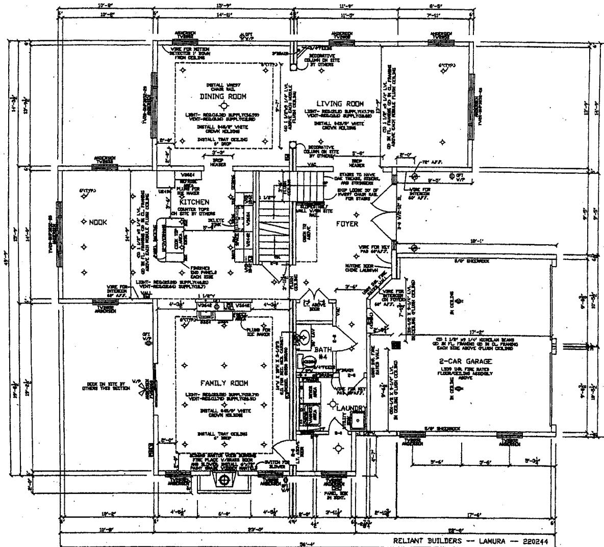
FIRST FLOOR PLAN SCALE 3/16" = 1'-0" 1/4" = 1'-0" CEILING
