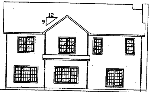
REAR ELEVATION SCALE 3/16" = 1'-0"
