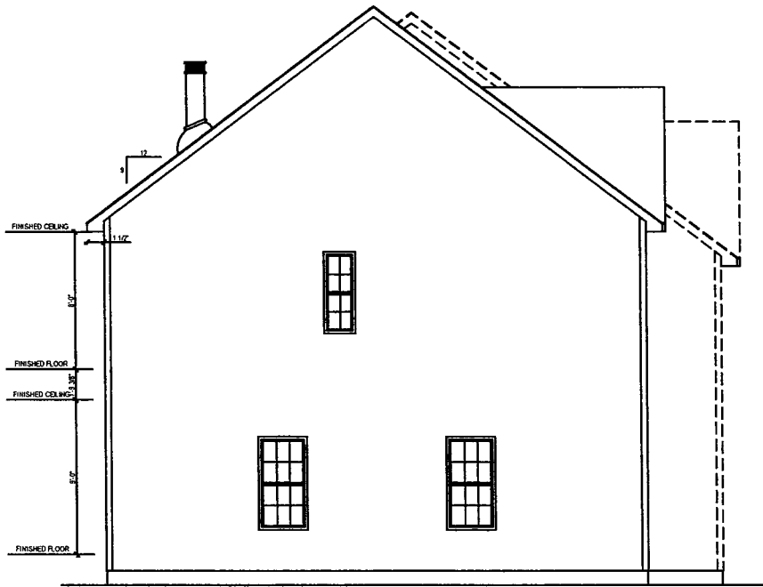
LEFT ELEVATION
