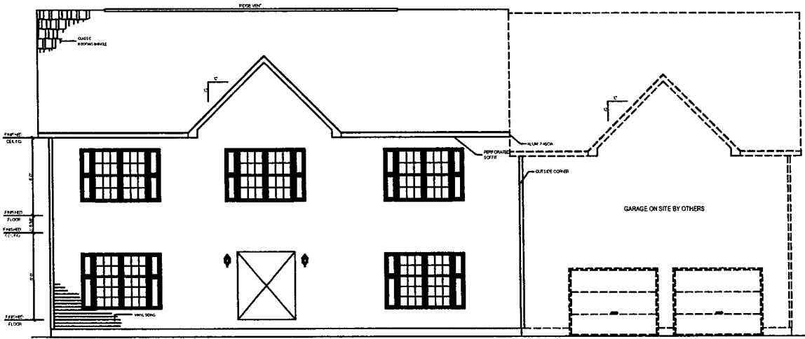
FRONT ELEVATION
