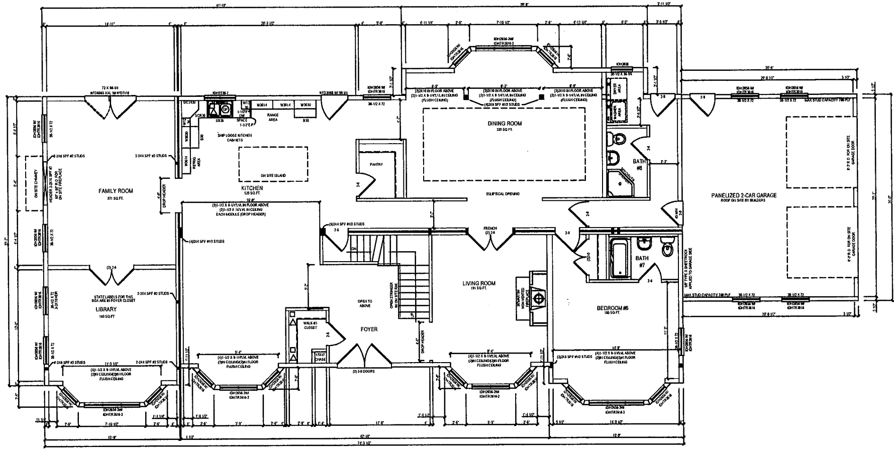
FIRST FLOOR PLAN 9'-0" CEILINGS
